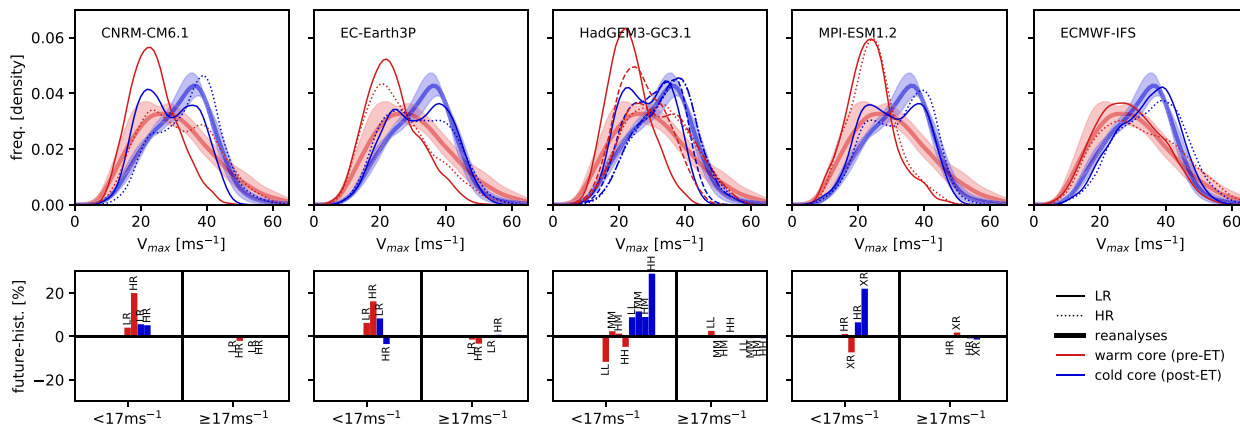
FIG. 11. As in Fig. 10, but for fully coupled simulations.
